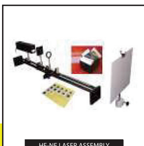
HE-NE LASER ASSEMBLY WITH OPTICAL BENCH
